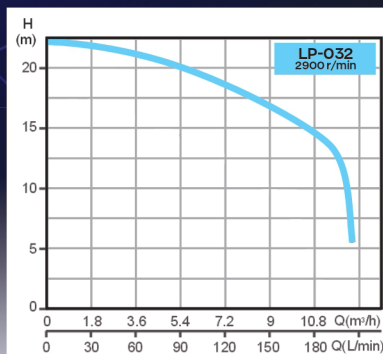
Performance Curve
