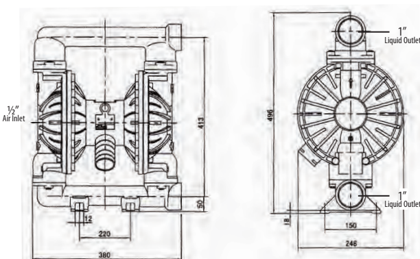
Installation Dimension
